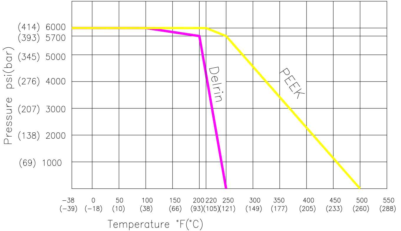
Pressure / Temperature Chart: CRS329VHPS & CRS429VHPS 6,000 psi Ball Valve
