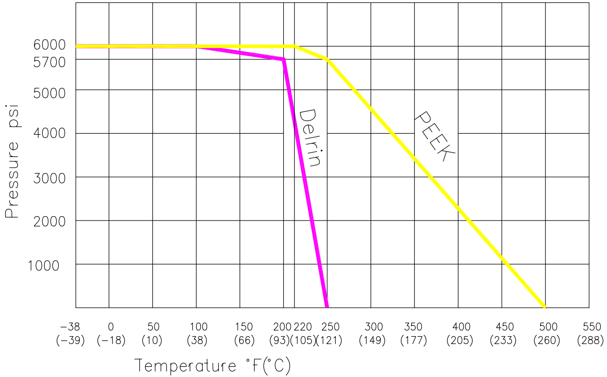
Pressure / Temperature Chart: CRS329VHPS & CRS429VHPS 6,000 psi Ball Valve
